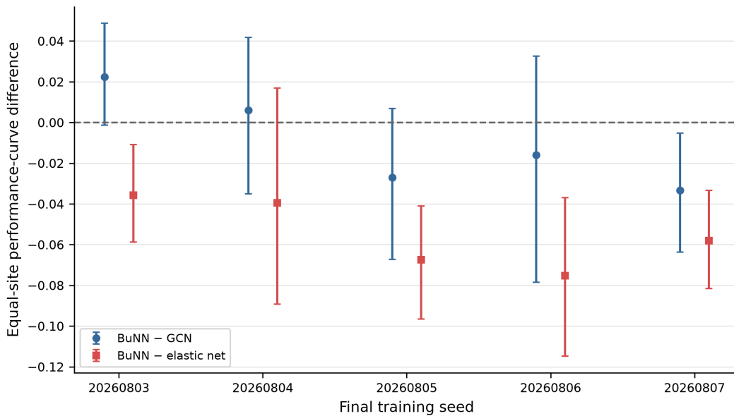
Figure 7: BuNN–GCN contrast across the five fixed final training seeds. Variation across seeds shows that the small average difference is sensitive to optimization randomness.
