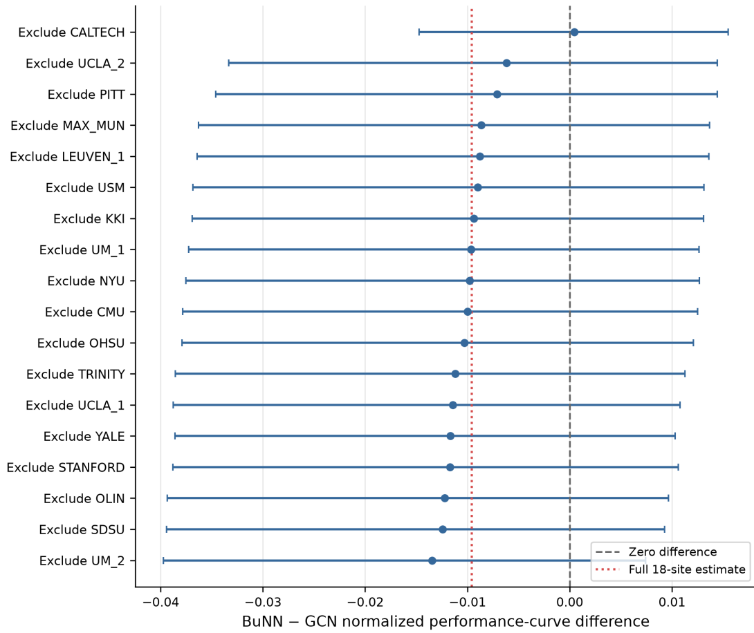
Figure 6: Leave-one-site influence on the BuNN–GCN curve contrast. This analysis tests whether the confirmatory average is driven by a single site; it does not create 18 independent replications.
