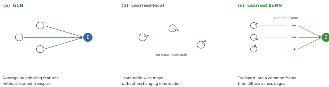
Figure 3: Computational distinction among GCN aggregation, the learned-local capacity control, and learned bundle transport. The schematic does not represent biological signal flow.
